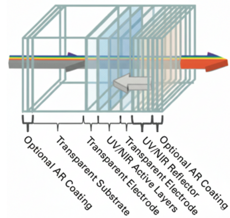
Fig. 2. Internal structure of TSC [19]
