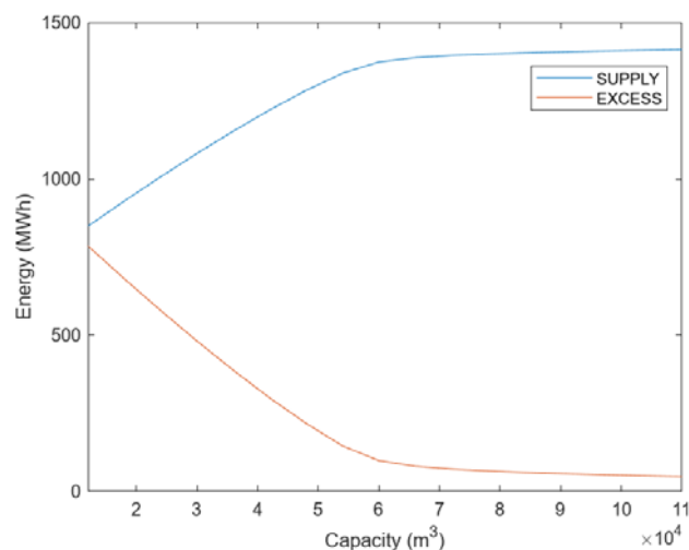
Fig. 7. Enlarged view of Figure 6, focusing on the initial saturation zone.
