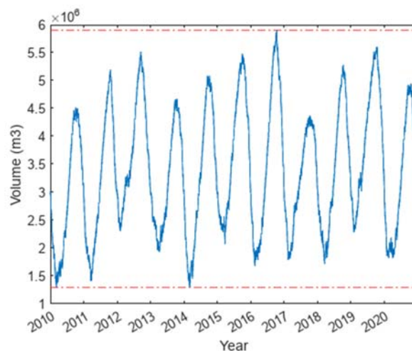
Fig. 3. Stored water volume for a full simulation.
