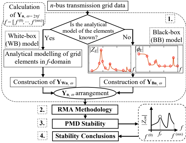
Fig. 4. Flowchart of RMA-based PMD stability criterion.
