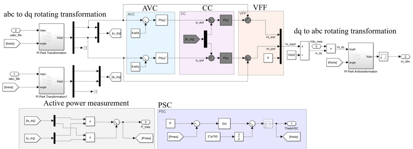
Fig. 1. MATLAB/Simulink model of the control Scheme 2 (PSC + AVC + CC strategy) of the GFM VSC.
