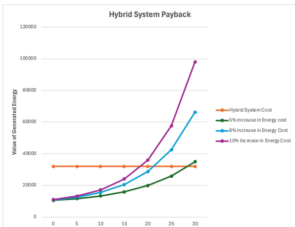
Figure 13 Hybrid system payback scenarios
