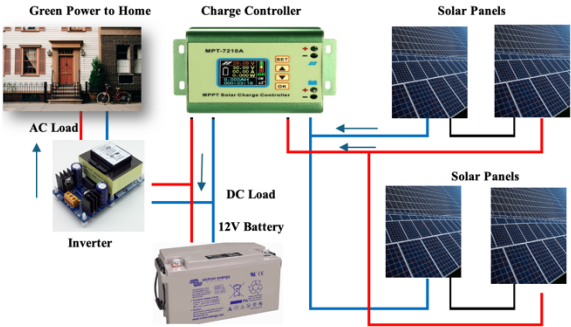
Figure 6: Power System Installation Diagram – Solar Power
